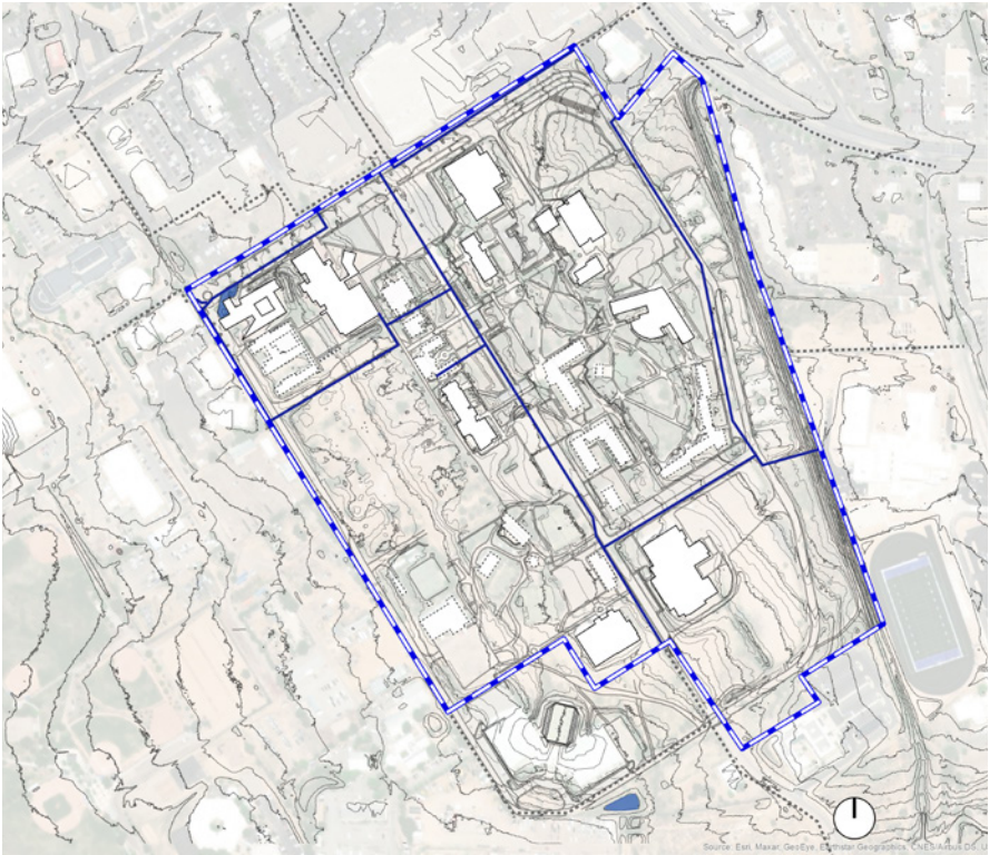
Existing Potable Water
